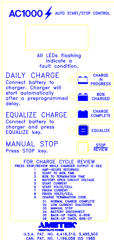
Figure 5-1 Status LEDs and Trouble Chart
